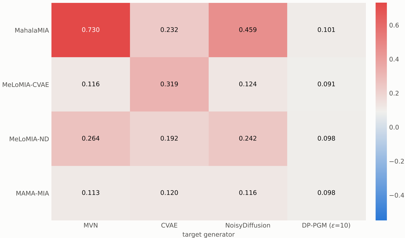
TPR @ 10% FPR — COMBINED
