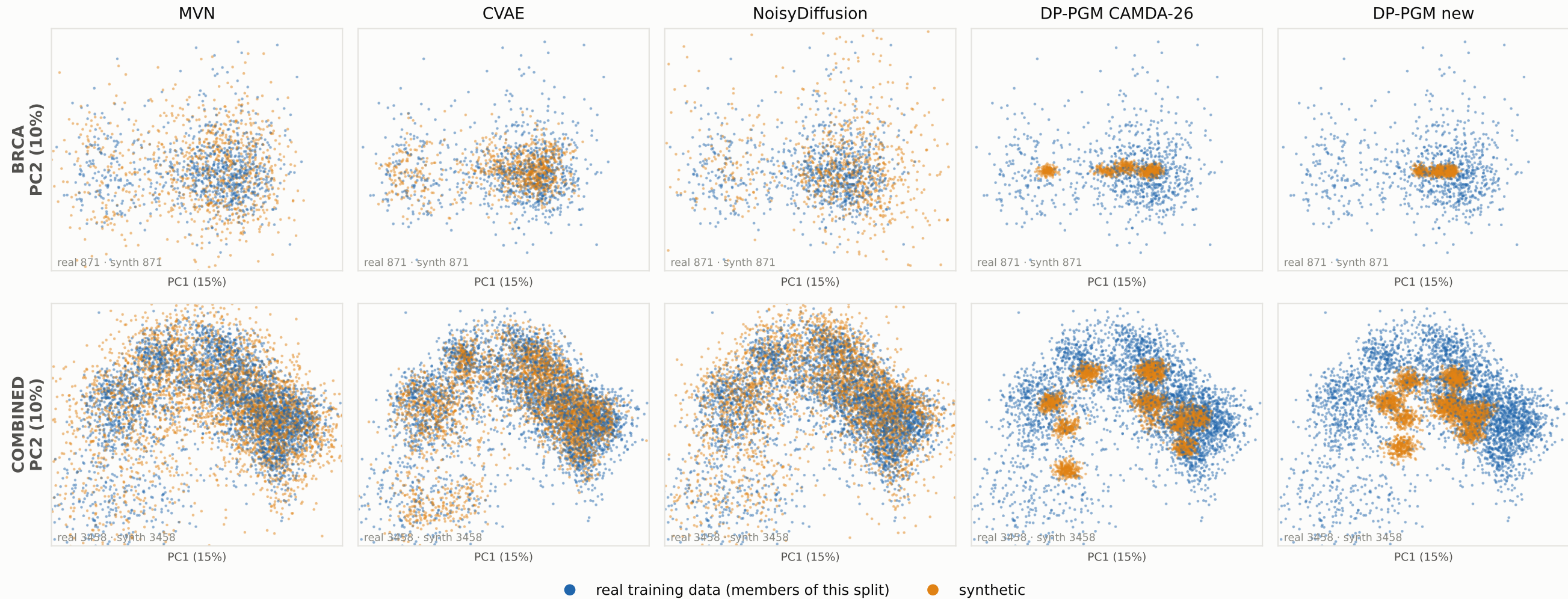
PCA fitted on the real training data, real vs synthetic, split 1 ( \epsilon = 10 for both DP-PGMs)
