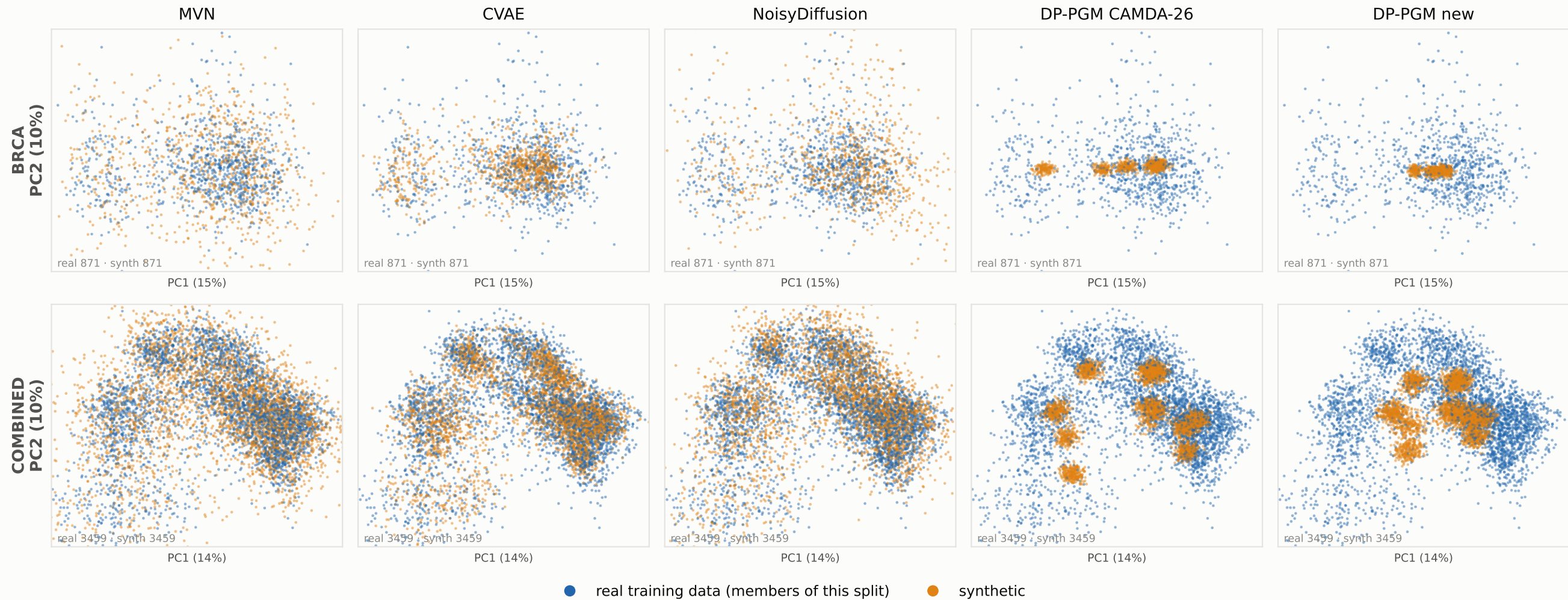
PCA fitted on the real training data, real vs synthetic, split 4 ( \epsilon = 10 for both DP-PGMs)
