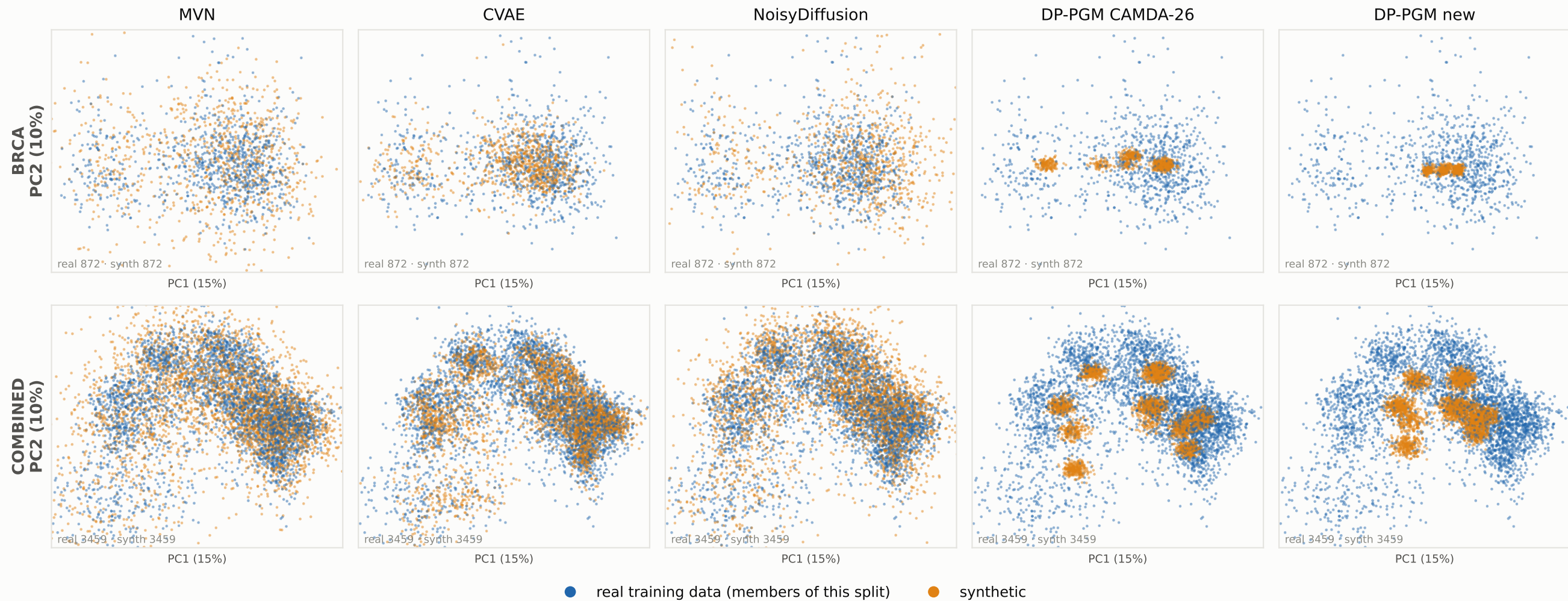
PCA fitted on the real training data, real vs synthetic, split 5 ( \epsilon = 10 for both DP-PGMs)
