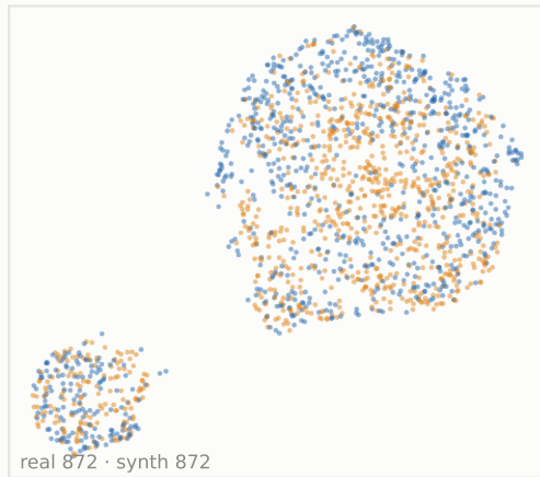
UMAP, real vs synthetic, split 5 ( \epsilon = 10 for both DP-PGMs)
