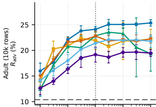
Random Forest
