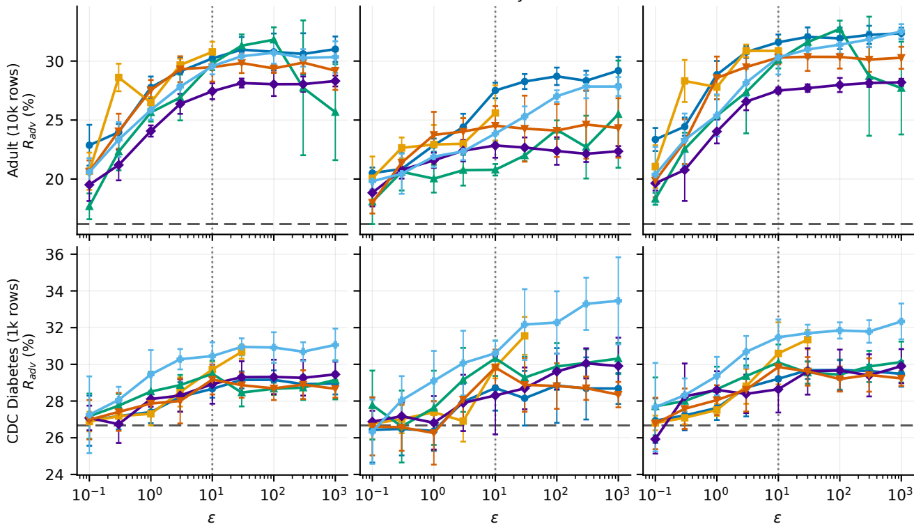
Random Forest
