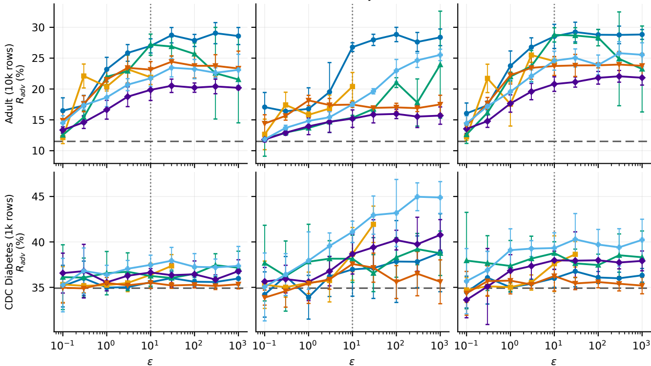
Random Forest
