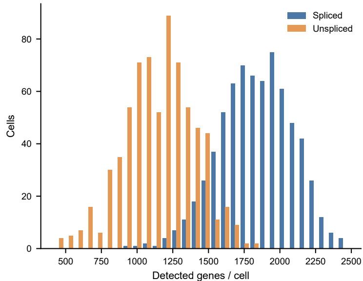
Splice detection
