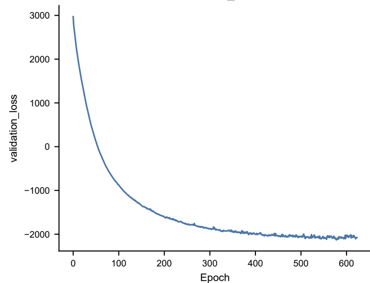
validation_loss
