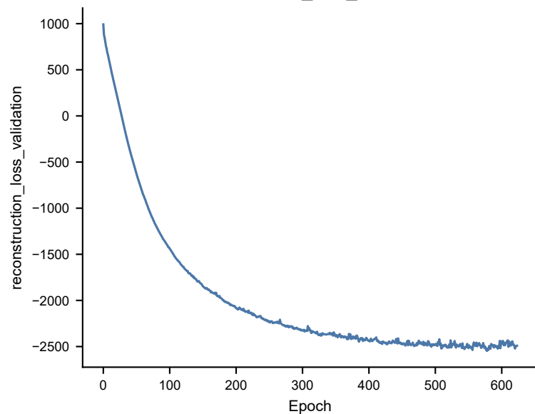
reconstruction_loss_validation
