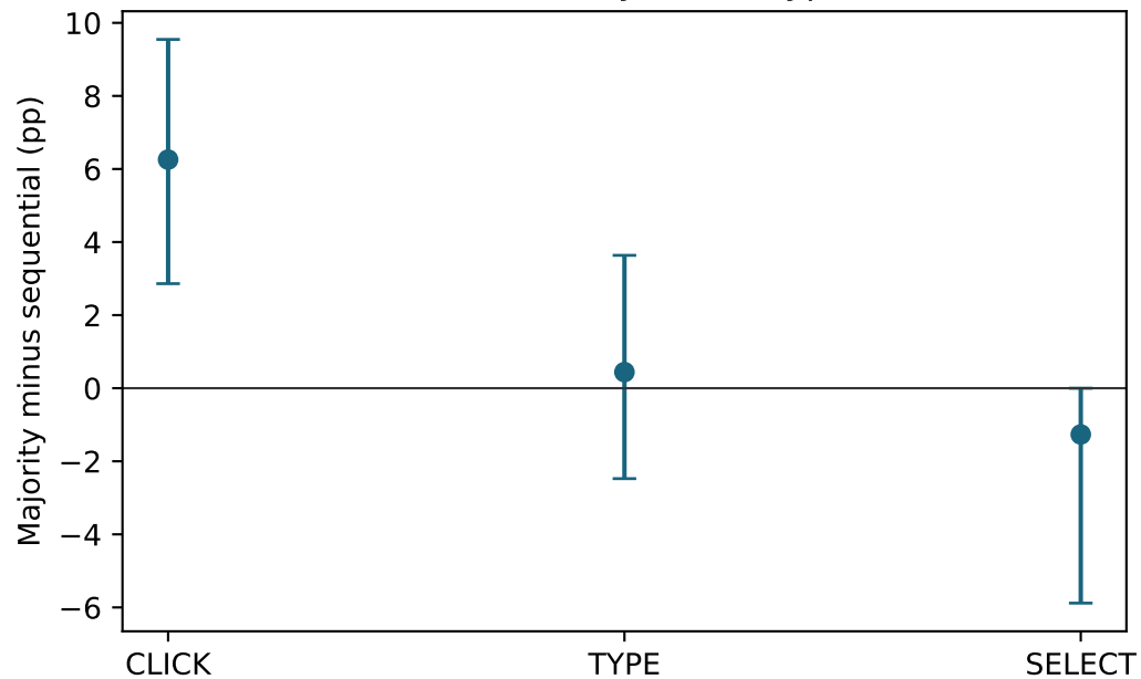
Mind2Web by action type
