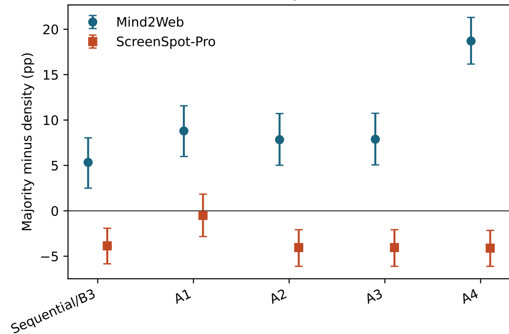
C-uni: action-space reversal
