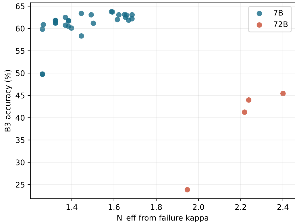
Effective sample size
