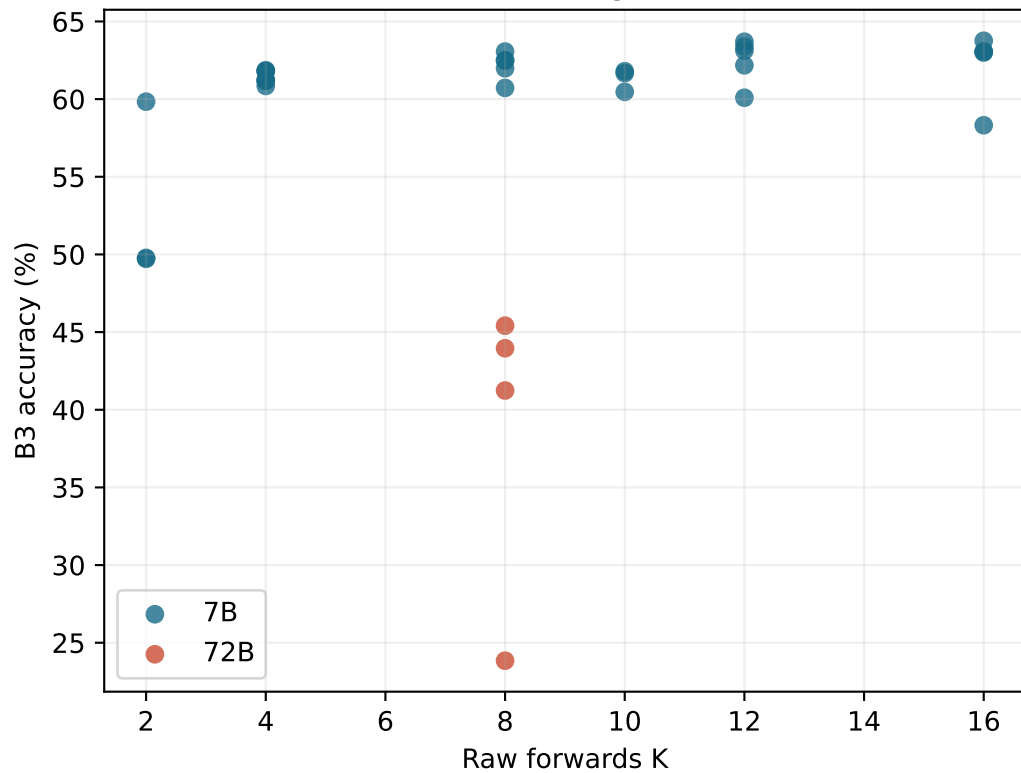
Raw budget
