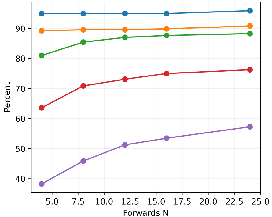
Candidate pass@N
