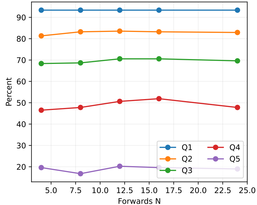
B3 accuracy
