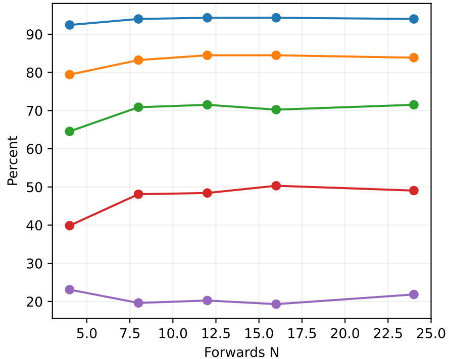
M1 accuracy
