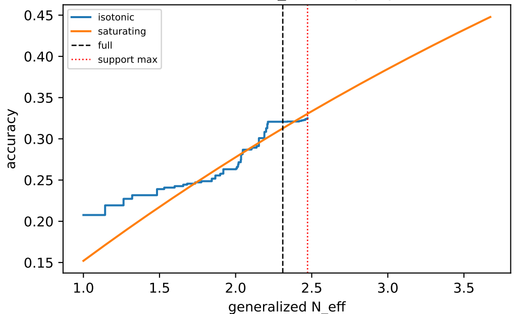
mind2web/C_self / majority
