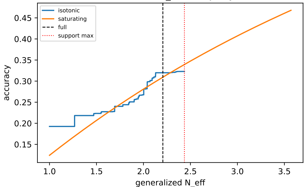
mind2web/C_cond / majority
