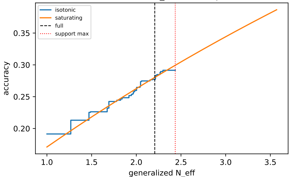
mind2web/C_cond / density
