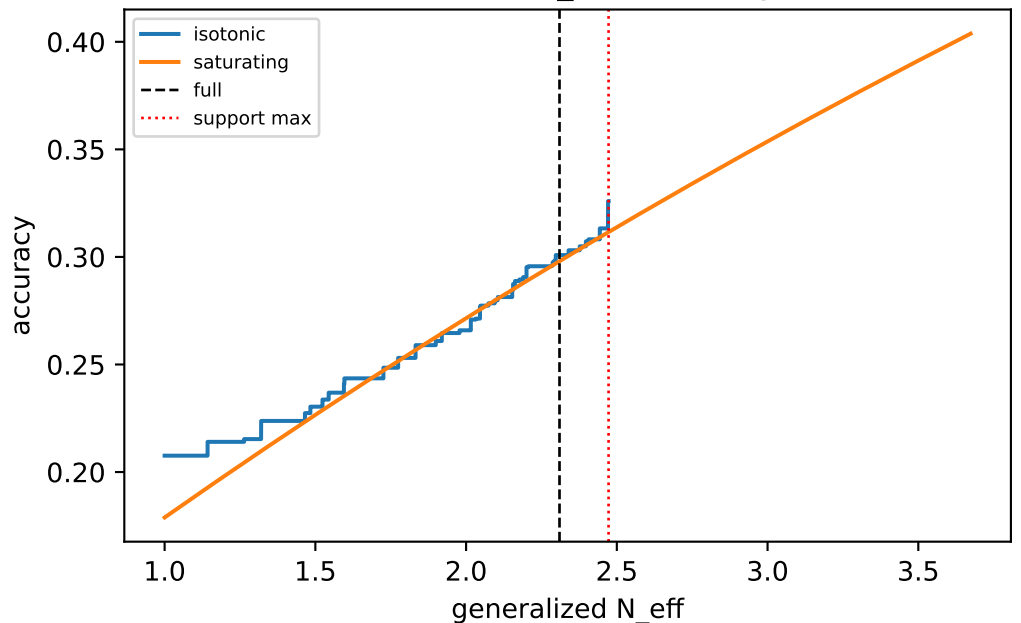
mind2web/C_self / density
