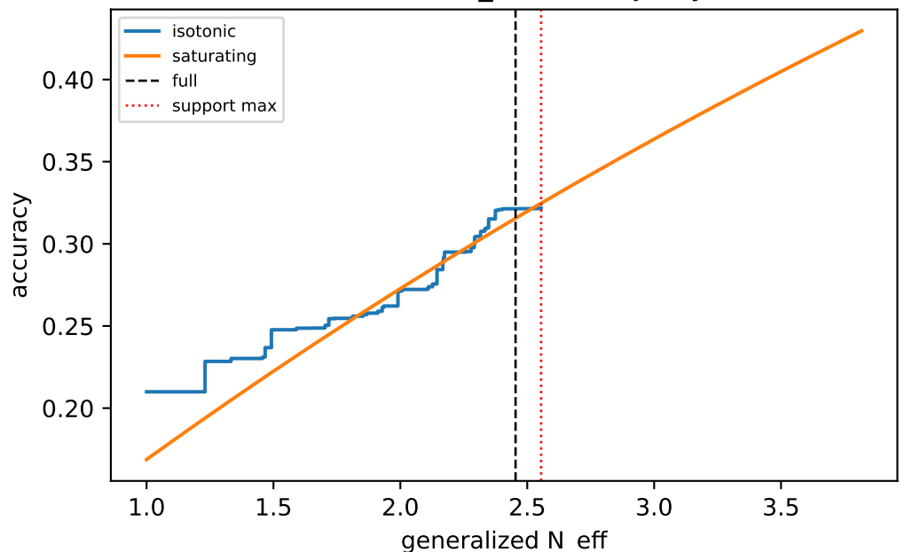
mind2web/C_rand / majority
