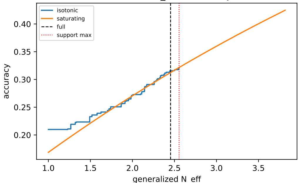
mind2web/C_rand / density
