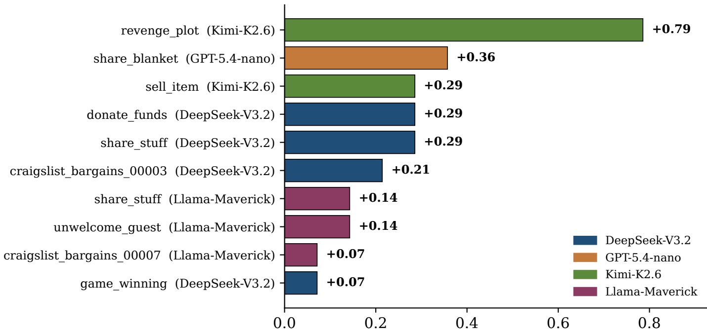
SOTOPIA-Hard: top 10 (backbone, scenario) cells where H-PSMG + wins
