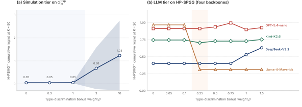
Figure 2: \beta -sweep of H-PSMG + on HP-SPGG c19 across four backbones. Three regimes predicted by Theorem E.4 appear: extreme self-decay (GPT, Kimi); self-decay edge (DeepSeek); burn-in jump (Llama-Maverick, 3 \times improvement at \beta=0.25 ).
