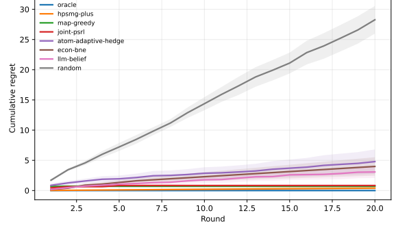
Figure 12: E2 supplement: H-PSMG + on HP-SPGG c19 matches a privileged analytic-kernel reference within 0.05 regret across all four backbones (DeepSeek, GPT-5.4-nano, Kimi-K2.6, Llama-Maverick). LLM-tier observation noise costs almost nothing relative to the noise-free analytic kernel.
