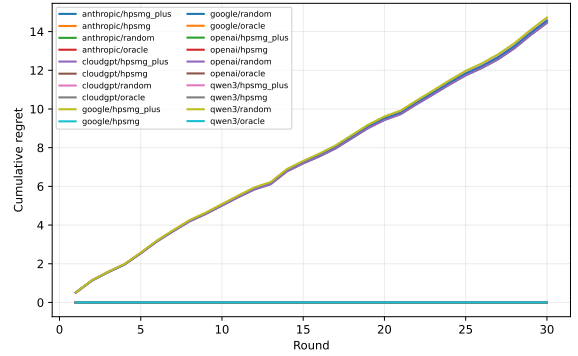
Figure 13: E3 supplement: cross-provider H-PSMG + rollouts on HP-SPGG, in which the n=3 agent slots are populated by two distinct backbones. The regret ordering across baselines is preserved, evidencing robustness to backbone mixing and ruling out single-provider bias.
