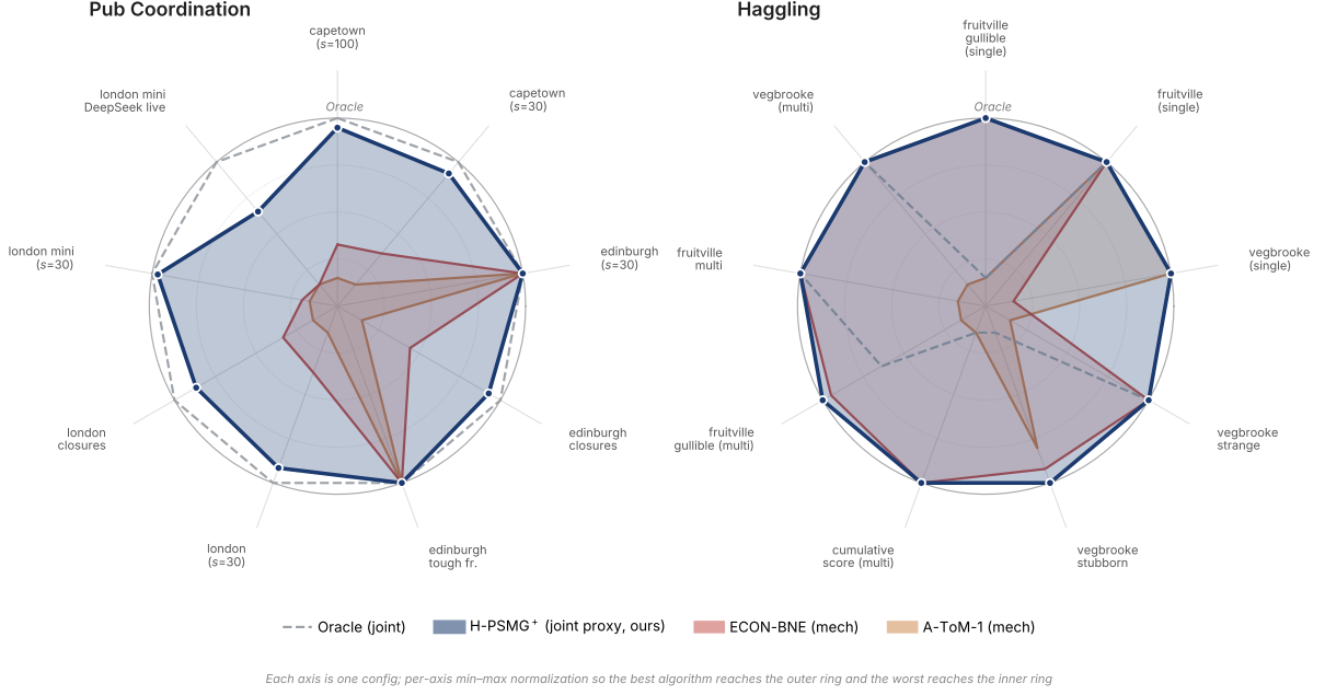
Figure 5: Concordia results. Left : Pub Coordination, 9 axes (7 village configs at s=30 , one at s=100 , one DeepSeek-V3.2 live LLM rollout at s=5 ). Right : Hagglng, 9 axes spanning 5 single-item and 4 multi-item configs at s=30 . Each axis is per-axis min-max normalised so the best of four algorithms reaches the outer ring; oracle is dashed and may sit inside the ring because H-PSMG + can strictly exceed oracle on focal score. H-PSMG + (joint proxy) fills nearly the full Pub Coordination polygon and wins or ties on every Hagglng axis.
