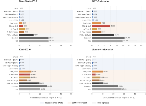
Figure 1: HP-SPGG cumulative Bayesian regret at K=20 across four LLM backbones (5 seeds, calibration c19). Three families: Bayesian type-aware (blue), LLM-coordination (warm), type-agnostic (gray). The H-PSMG family attains the lowest non-oracle regret on every backbone, separating from the best LLM-coordination baseline by 6–12 \times and from the best type-agnostic baseline by over 25 \times .
