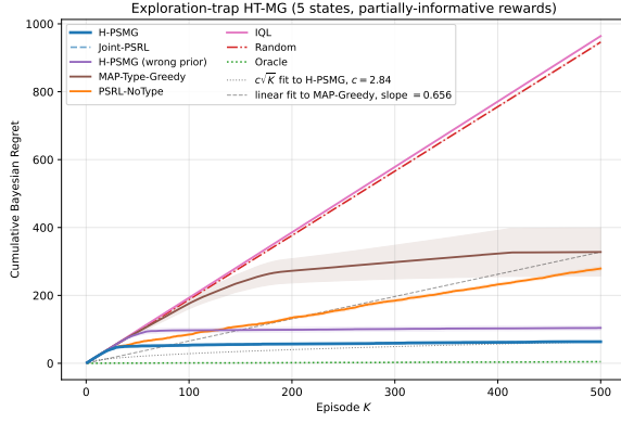
Figure 7: Analytic-kernel simulation of the exploration-trap game \mathcal{G}^* of Theorem E.3: cumulative Bayesian regret of H-PSMG, MAP-Type-Greedy, and PSRL-NoType under coupled randomness. MAP-Type-Greedy and PSRL-NoType both display the predicted \Omega(K) linear growth on the trap event; H-PSMG remains \tilde{O}(\sqrt{K}) .
