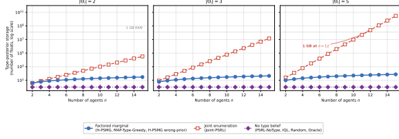
Figure 10: Storage saving of posterior decoupling: |\Theta|^n = |\Theta_i|^n for the joint posterior vs. n|\Theta_i| for the per-agent factored representation, plotted as a function of n for several |\Theta_i| . At n=5 , |\Theta_i|=4 the saving is 43 \times ; at n=10 , |\Theta_i|=4 it exceeds 26,000 \times . This is the analytic counterpart of the storage curve overlaid in the LLM-tier E3 result (Figure 4b).
