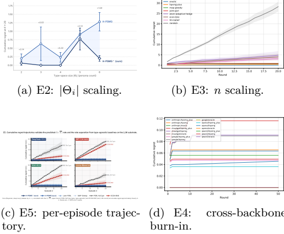
Figure 4: Consolidated empirical evidence for Theorems E.4 and E.3. (a) E2: bonus gap grows from +0.14 at |\Theta_i|=2 to +1.08 at |\Theta_i|=6 on Llama-Maverick, tracing the predicted \Omega(|\Theta_i|^n) -vs- O(1) envelope of Theorem E.4(ii). (b) E3: bonus benefit grows monotonically with n \in \{3, 4, 5\} while storage savings scale analytically as |\Theta_i|^n/(n|\Theta_i|) ( 43\times at n=5 ). (c) E5: per-episode cumulative-regret trajectories on HP-SPGG across four backbones; H-PSMG and H-PSMG + plateau at < 0.05 regret per episode within K \approx 5 (the \tilde{O}(\sqrt{K}) envelope of Theorem E.1) while PSRL-NoType grows linearly ( 0.50 – 0.93 per episode), realising the rate separation of Theorem E.3 with cumulative gap 11 – 30\times at K=20 . (d) E4: per-backbone burn-in episode K_{\text{conc}}^{0.9} matches the regime ordering of Figure 3. Cross-checks against the analytic kernel (E2-suppl) and against cross-provider rollouts (E3-suppl) appear in Appendix L.
