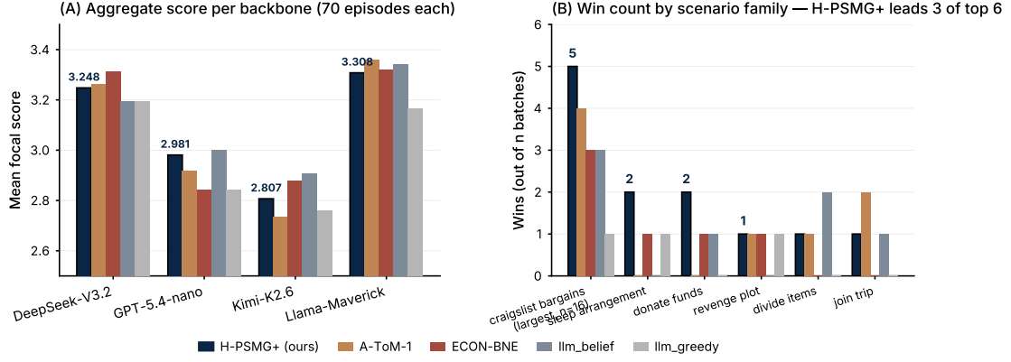
Figure 6: SOTOPIA-Hard results. (A) Aggregate mean focal score per (backbone \times baseline), 70 episodes per cell. H-PSMG + (deep navy, bold outline) stays within 0.1 of the leader on every backbone (numerical scores marked); the five baselines cluster in a 0.12-score envelope, indicating that out of scope no algorithm achieves a clear separation – consistent with the prior-factorisation lower bound. (B) Wins per scenario family across the 56 (backbone, scenario codename) pairs. H-PSMG + leads on the largest family craigslist_bargains (5/16) and on sleep_arrangement and donate_funds (2/4 each), ties on revenge_plot , and is competitive (1 win) on divide_items and join_trip .
