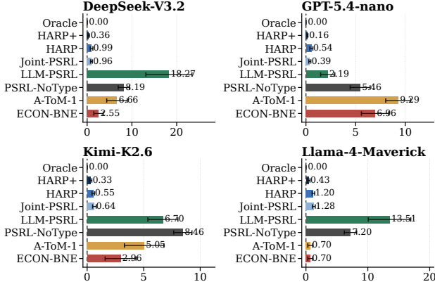
Cumulative Bayesian regret at K=20 (mean ± SEM; 10 common environments)
