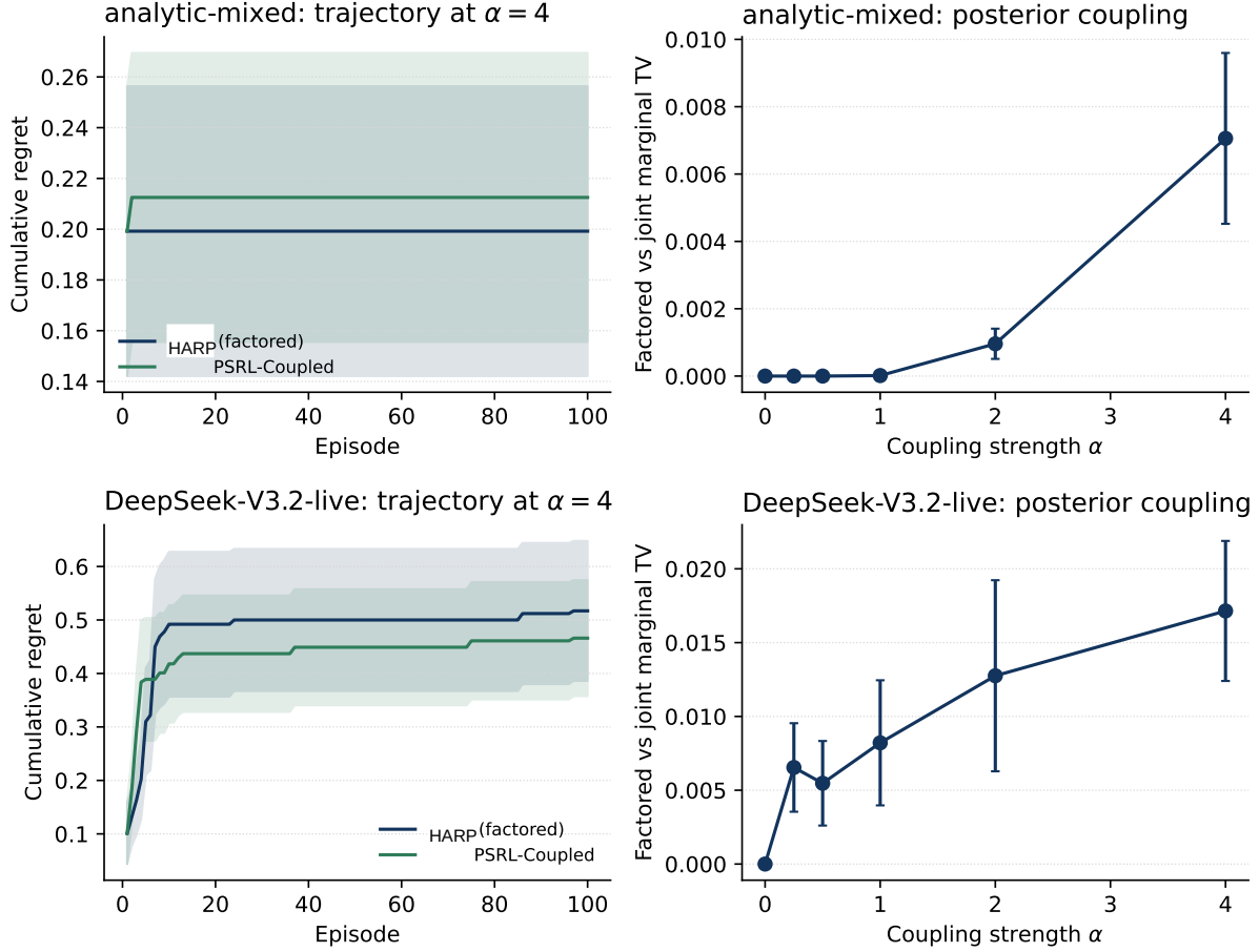
Figure 13: C4 reward-locality violation ( K=100 , 10 common environment seeds). Left: HARP and correctly specified Joint-PSRL regret trajectories at \alpha = 4 . Right: marginal TV between HARP’s factored posterior and a shadow exact-joint posterior on the same trajectory. Top is analytic; bottom uses all 324 live DeepSeek persona/player/action cells. Posterior coupling increases, but no regret disadvantage is detectable on this geometry.
