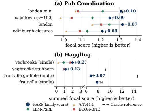
Figure 5: Focal-agent payoff on the Concordia substrates. (a) Pub Coordination , with oracle_joint as the reference. (b) Haggling , with the exact oracle_focal as the reference. Blue labels give the margin of HARP + in each configuration.
