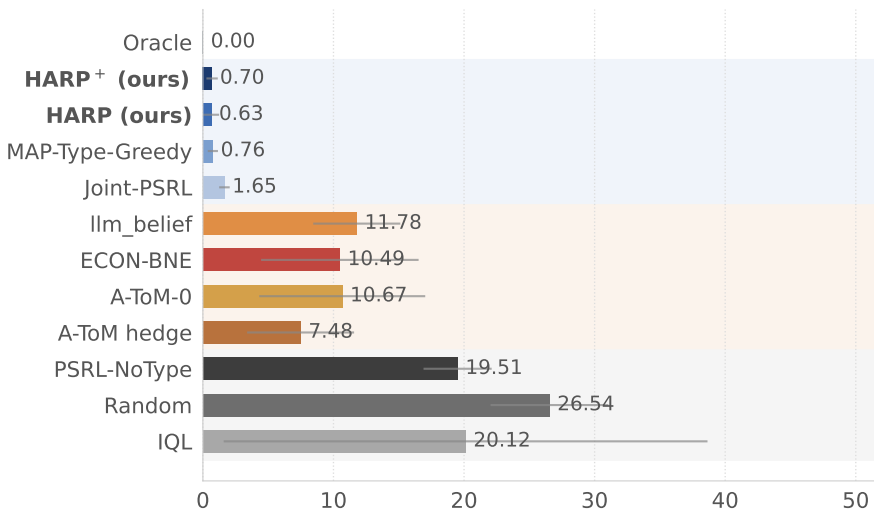
Kimi-K2.6
