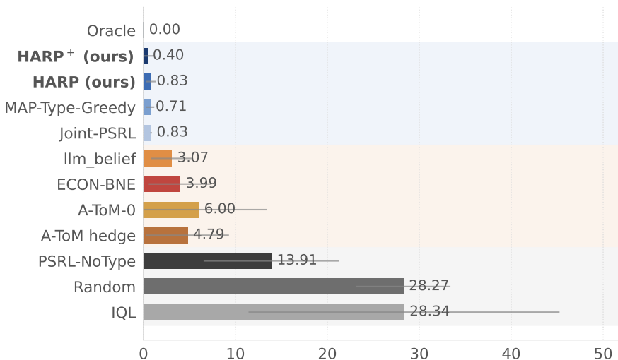
Kimi-K2.6
