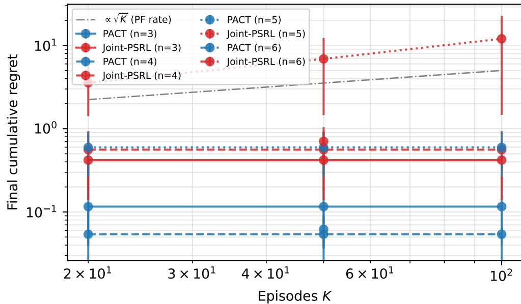
Regret vs K (shared_type, analytic)
