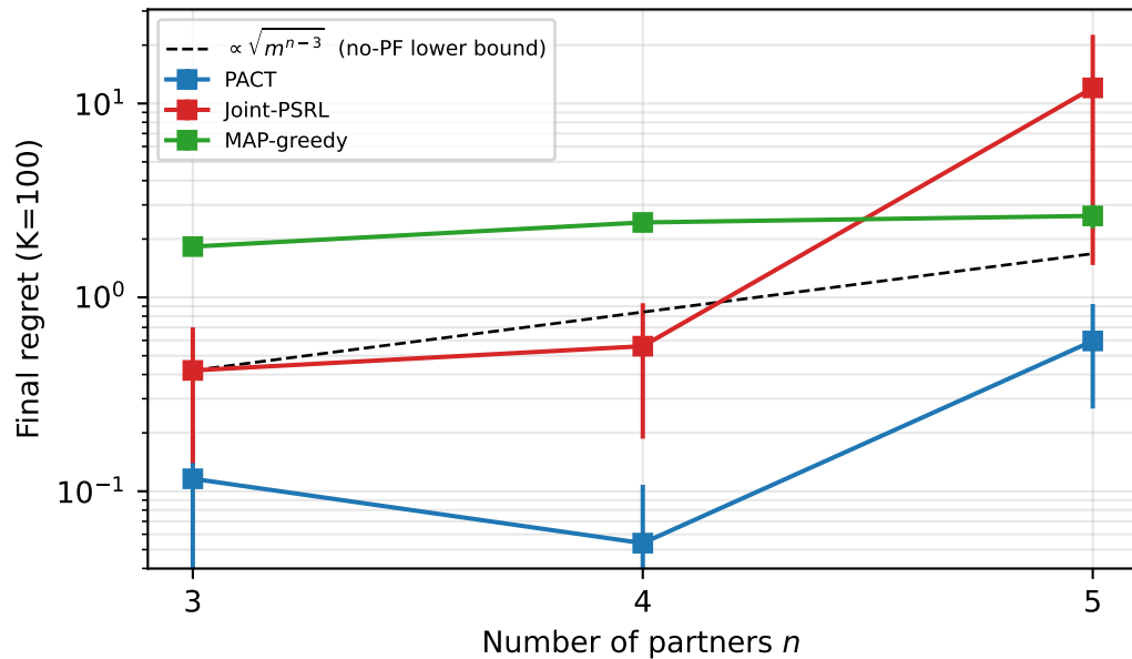
Regret vs n (shared_type, analytic)
