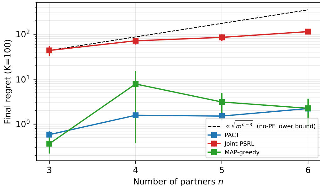
Regret vs n (shared_type, llama_maverick)
