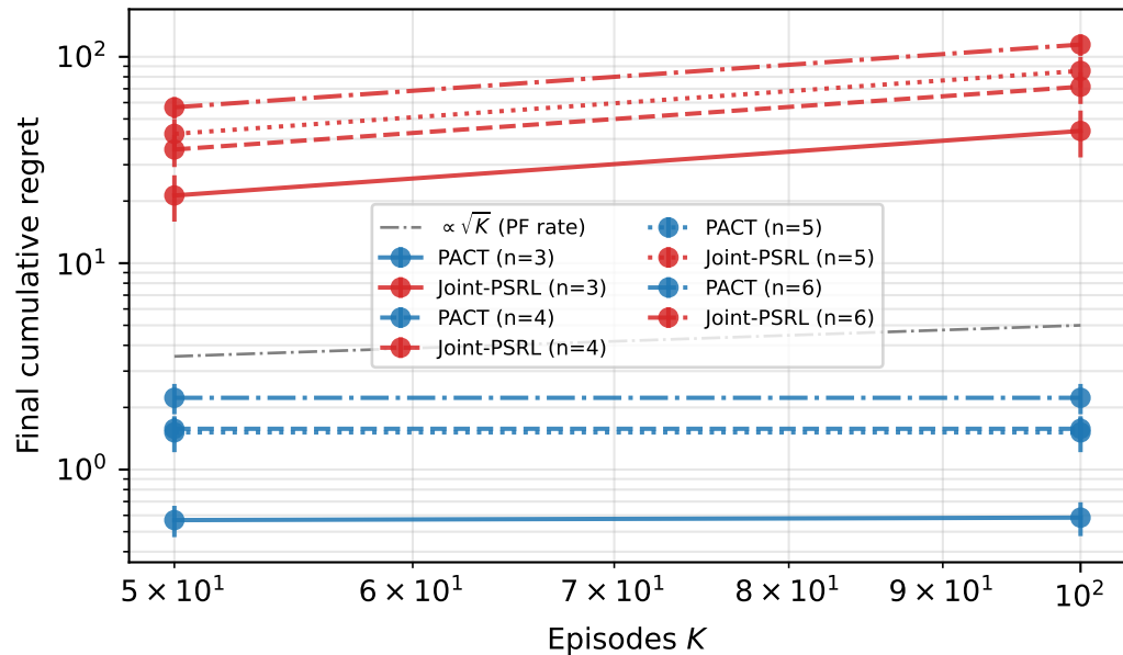
Regret vs K (shared_type, llama_maverick)
