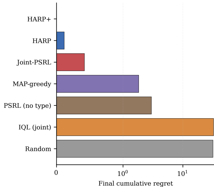
(b) Shared-type prior
