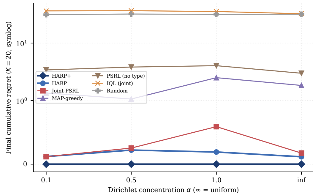
(a) Symmetric joint prior
