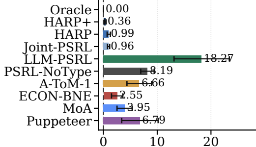
Kimi-K2.6
