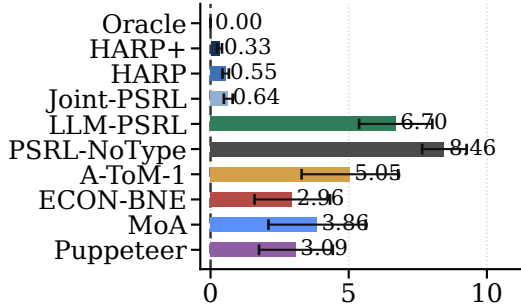
Kimi-K2.6
