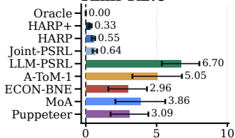
Kimi-K2.6
