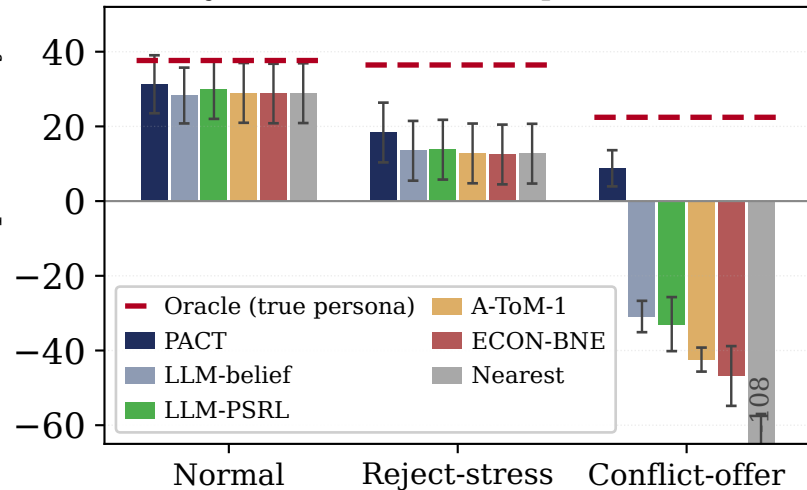
(a) Utility vs. baselines under persona-cost stress
