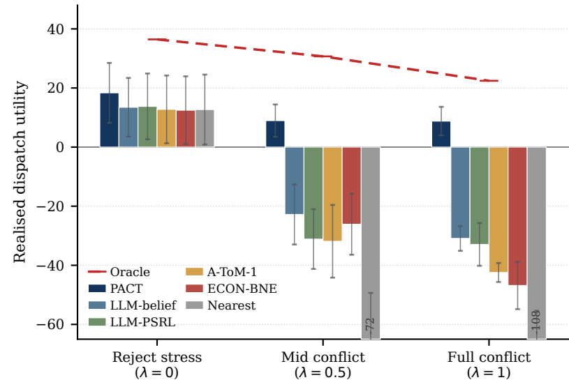
(a) Utility across conflict strength
