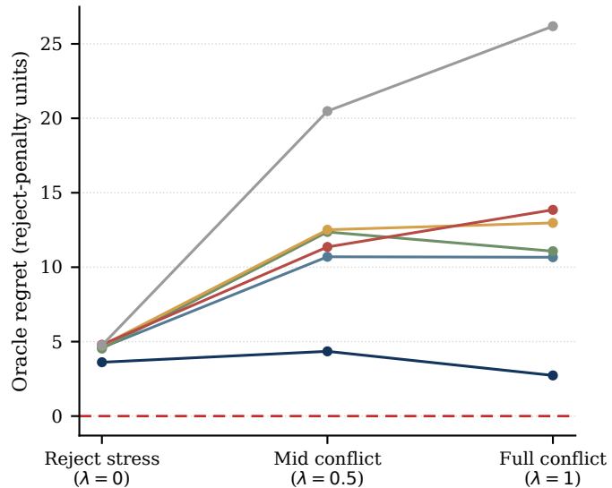
(b) Controlled stress continuum
