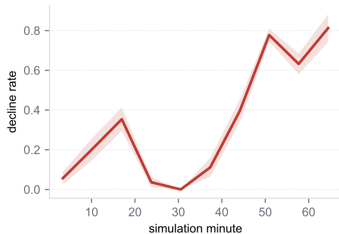
Observed decline rate
