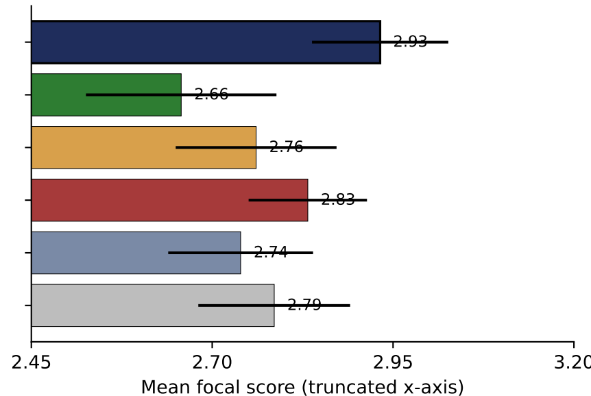
Revenge plot ( \Delta=+0.10 )
