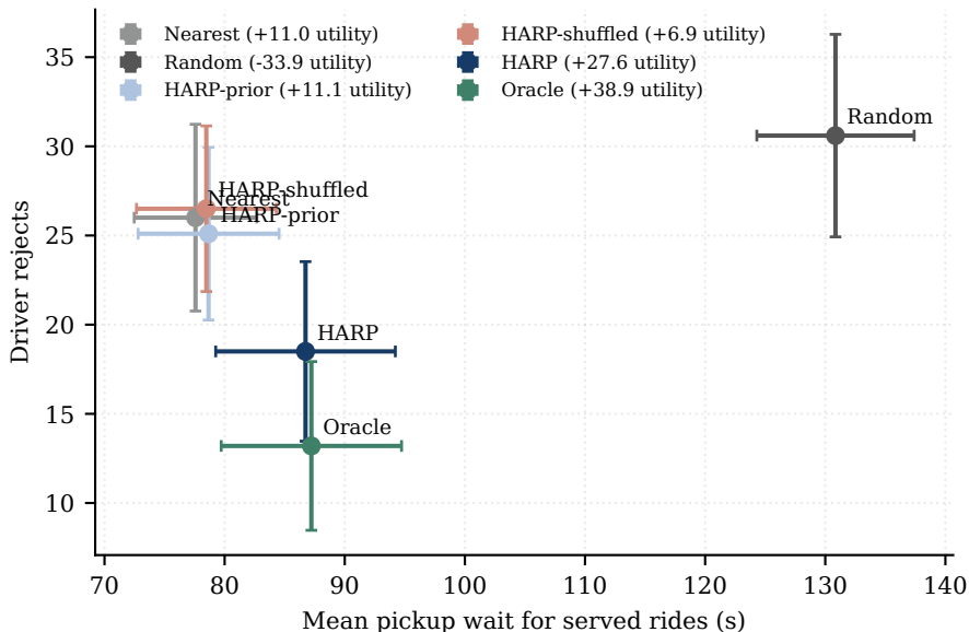
MaaSSim wait-reject trade-off
