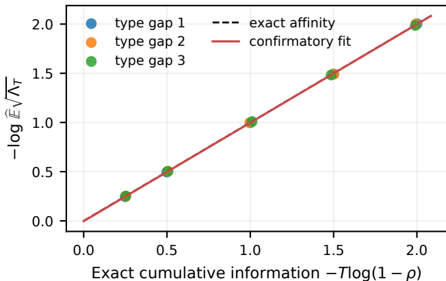
(c) Simultaneous-agent concentration
