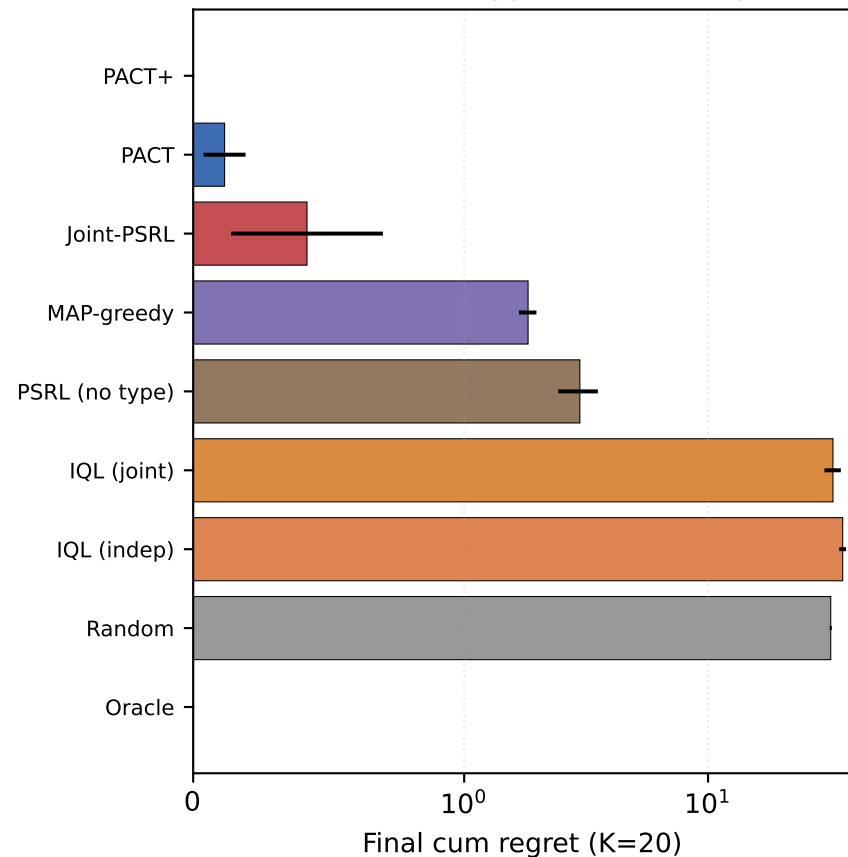
E-1.3b: shared-type structured prior
