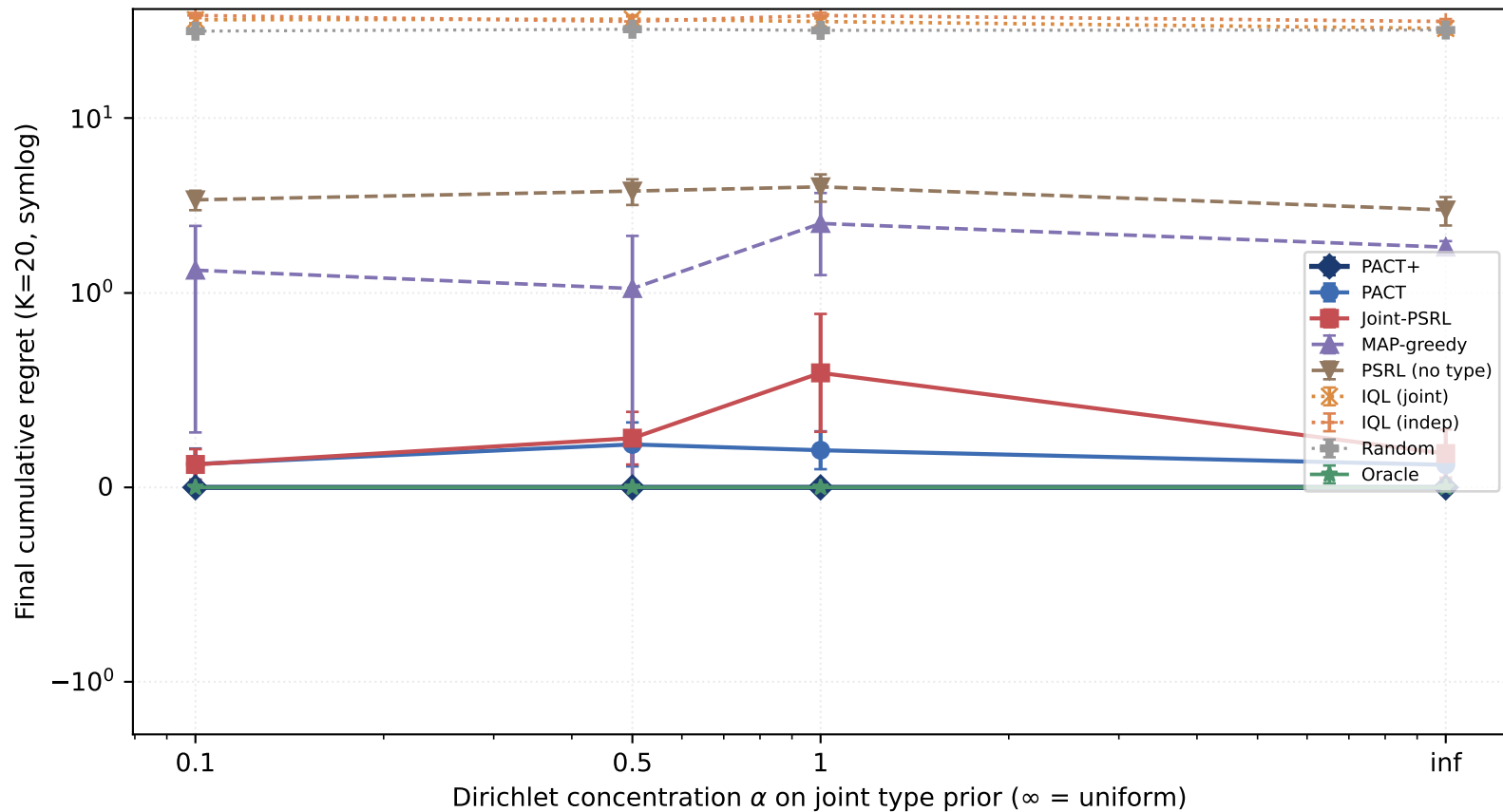
E-1.3a: symmetric Dirichlet joint prior on |\Theta|^n = 64 profiles (n=3)
