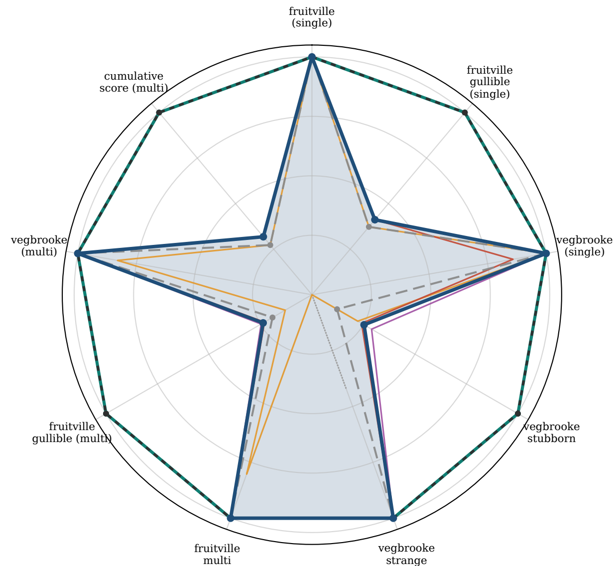
Haggling (Dual Oracle)
