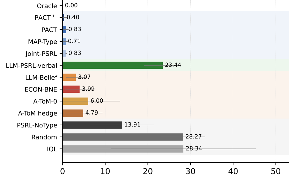
Kimi-K2.6
