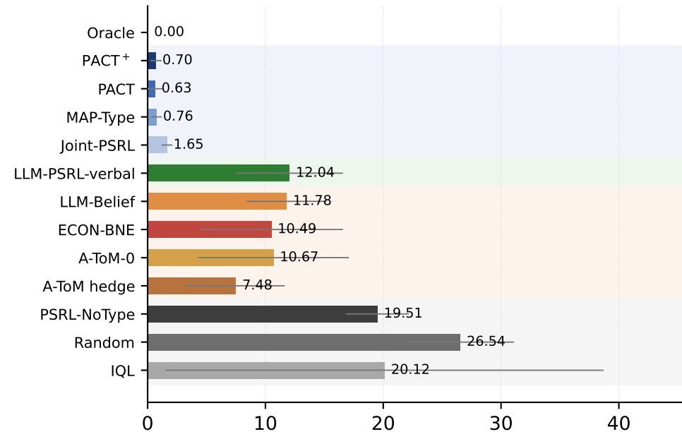
Kimi-K2.6
