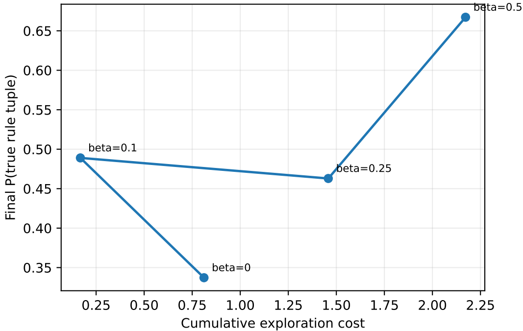
PACT+ probe-cost trade-off
