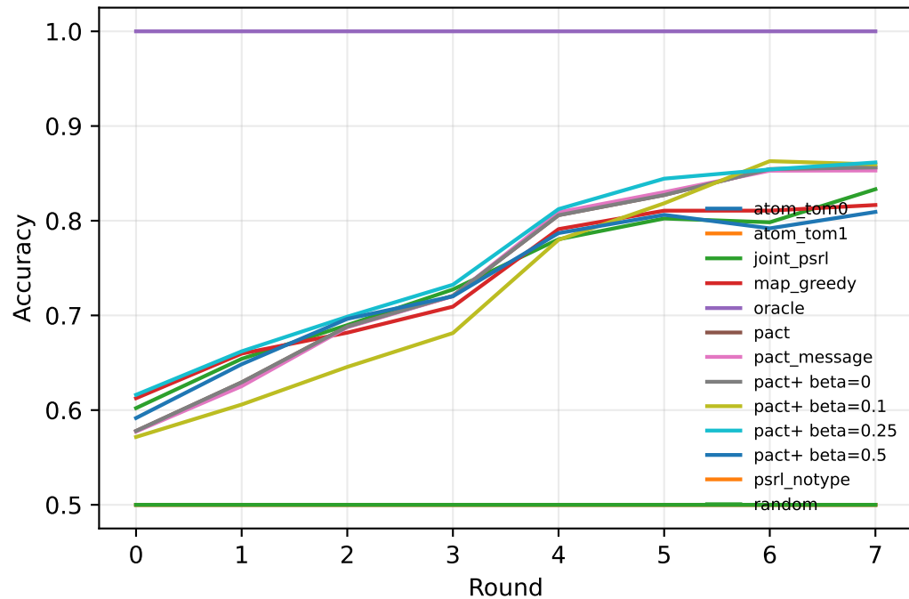
Rule-marginal accuracy
