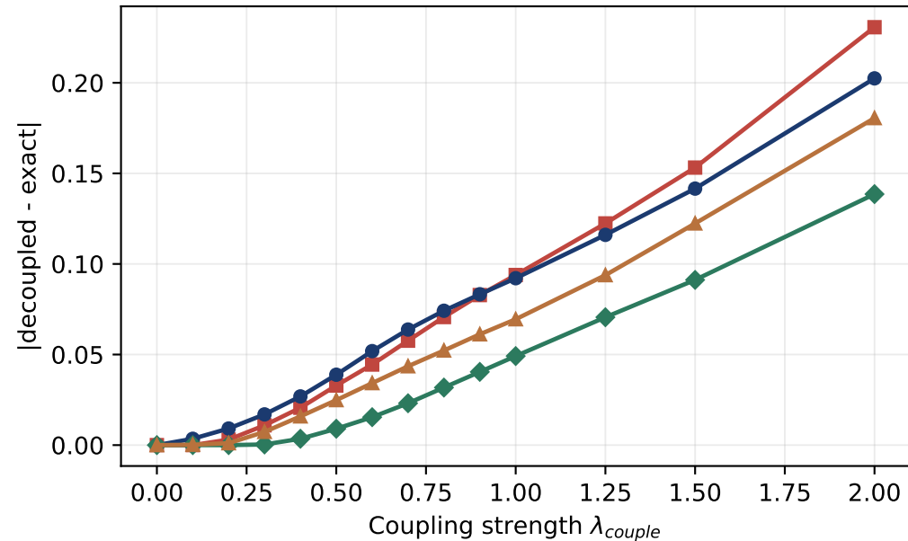
Decoupled value error
