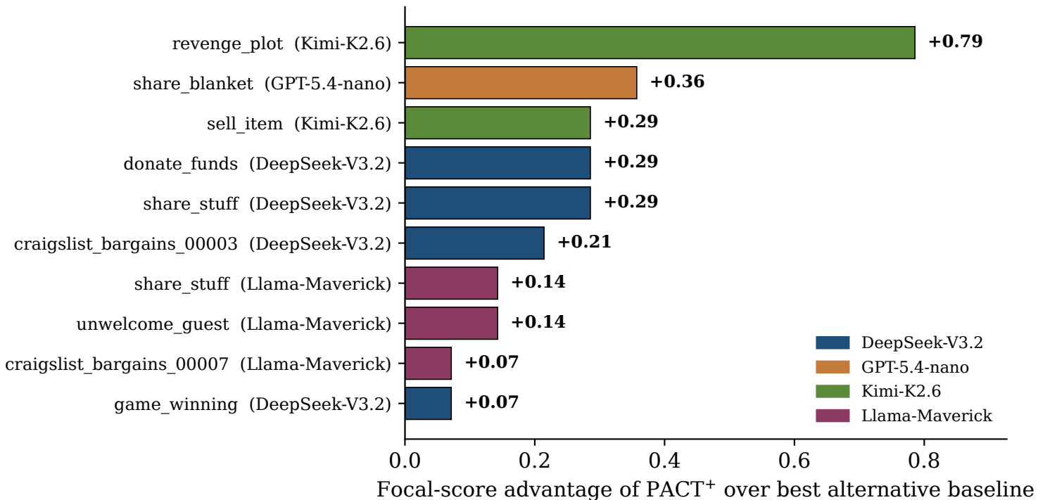
SOTOPIA-Hard: top 10 (backbone, scenario) cells where PACT + wins
