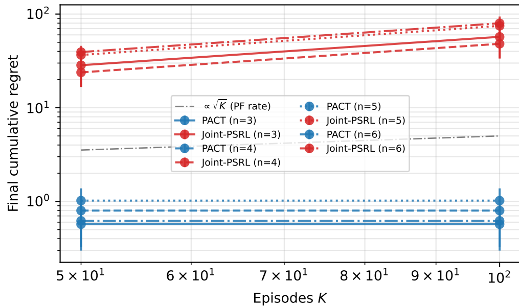
Regret vs K (shared_type, deepseek)
