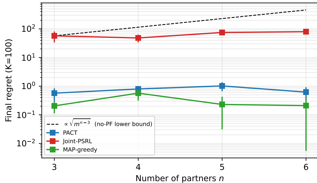
Regret vs n (shared_type, deepseek)
