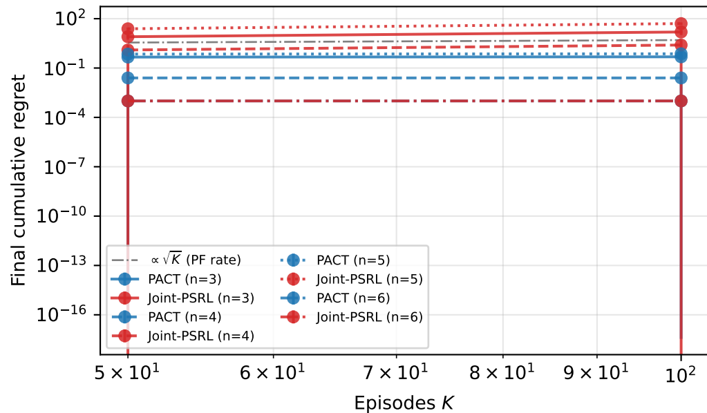
Regret vs K (shared_type, gpt5_nano)
