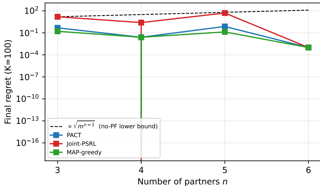
Regret vs n (shared_type, gpt5_nano)
