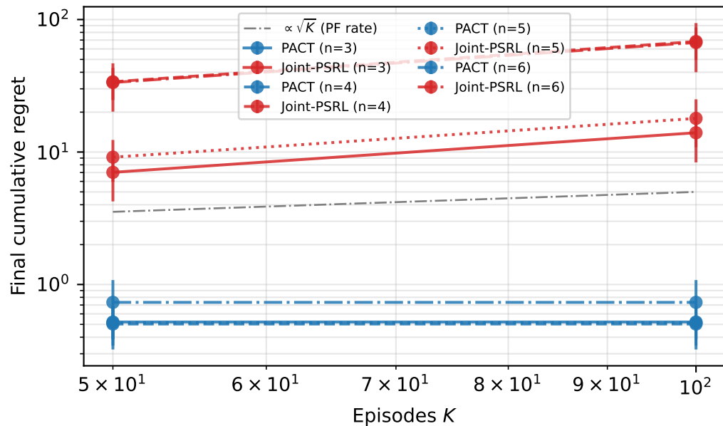
Regret vs K (shared_type, kimi_k2)
