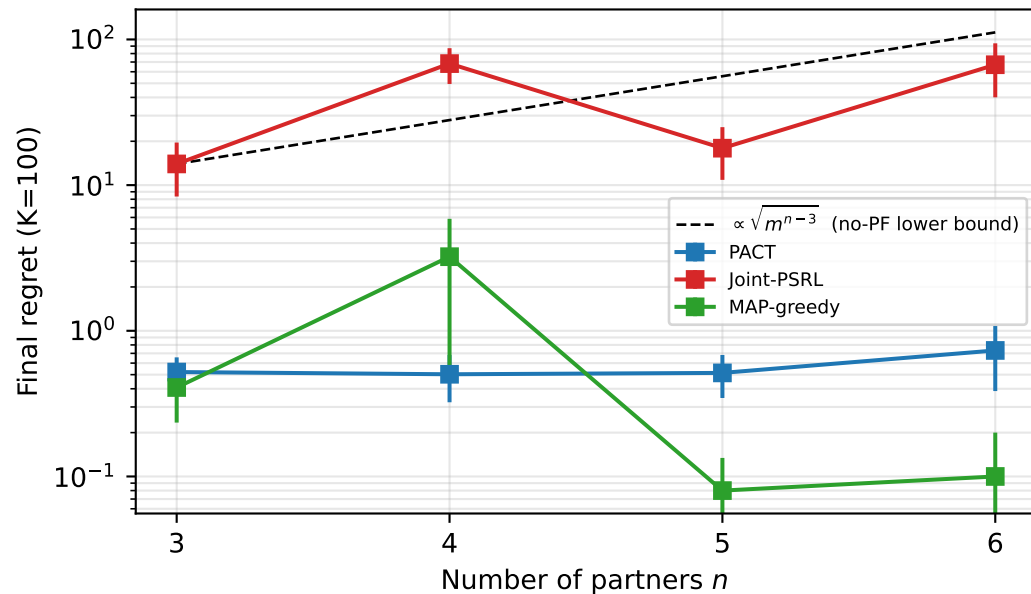
Regret vs n (shared_type, kimi_k2)
