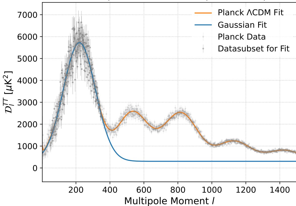
Power Spectrum of CMB Temperature Map
