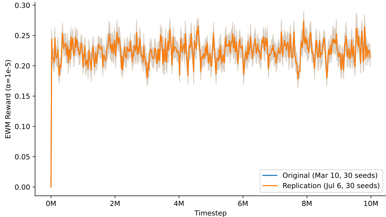
Search-Oracle on ForagaxBig-v5: Original vs Replication
