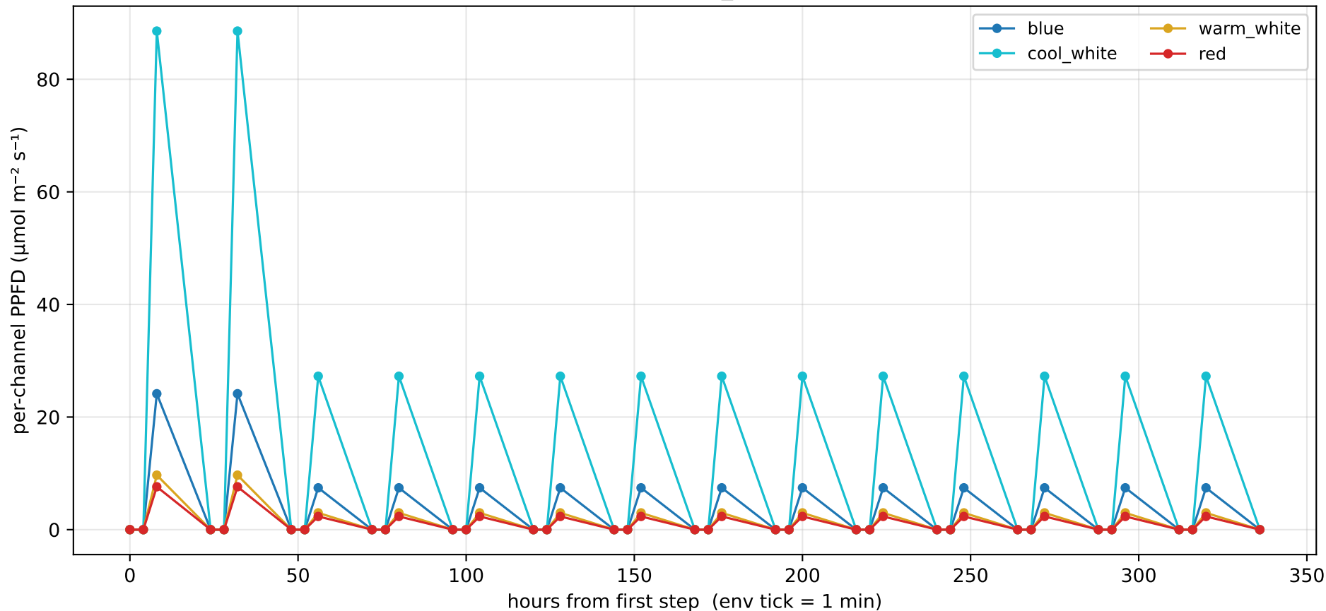
Z4 differential explore (adaptive) — actions emitted via main_real path (14 sim-days at 1-min env steps, 20160 total)
