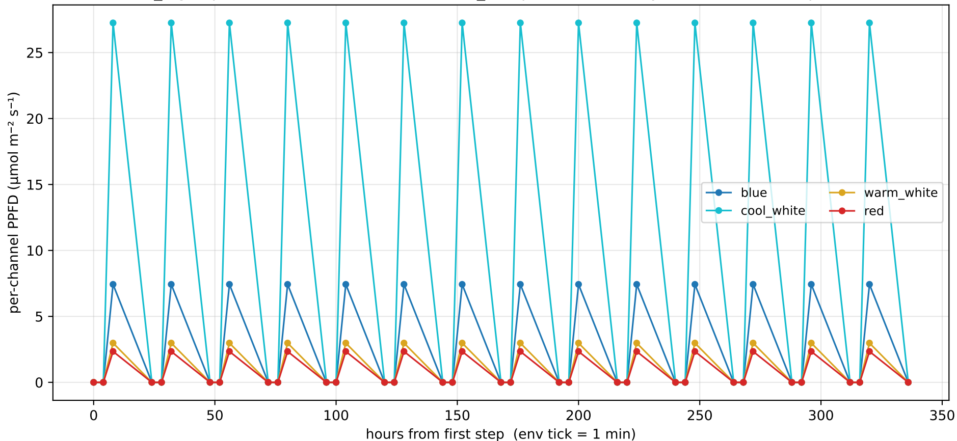
Z2 masked_log exploit — actions emitted via main_real path (14 sim-days at 1-min env steps, 20160 total)
