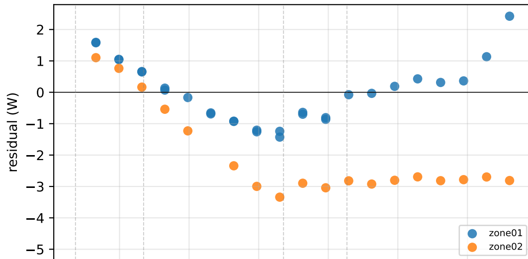
linear (2p) zone01 RMSE=0.97 W
