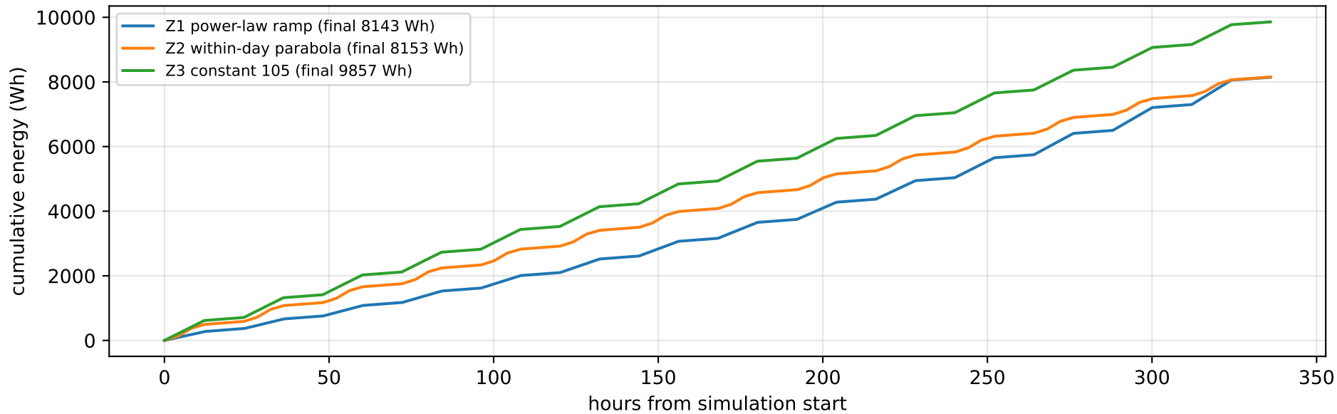
Cumulative lights-on energy over the 14-day window
