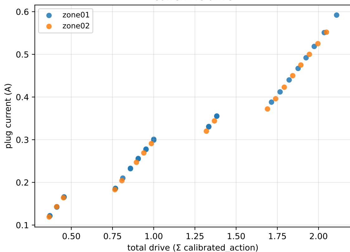
Current vs drive
