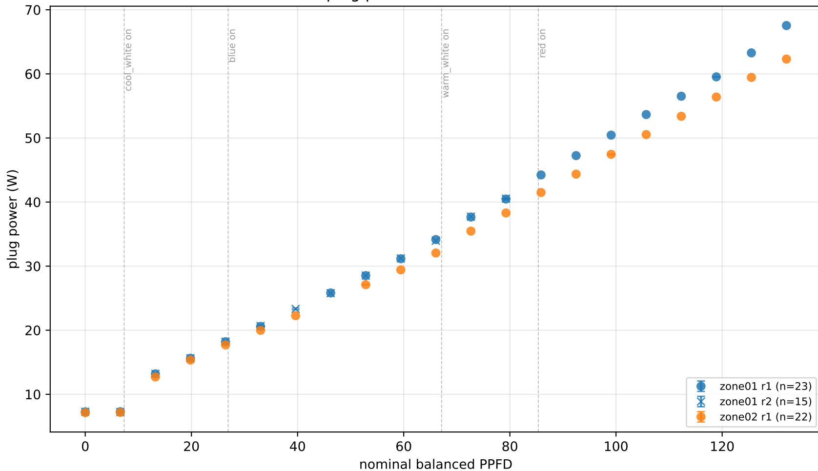
E18/P0.1: plug power vs nominal balanced PPFD
