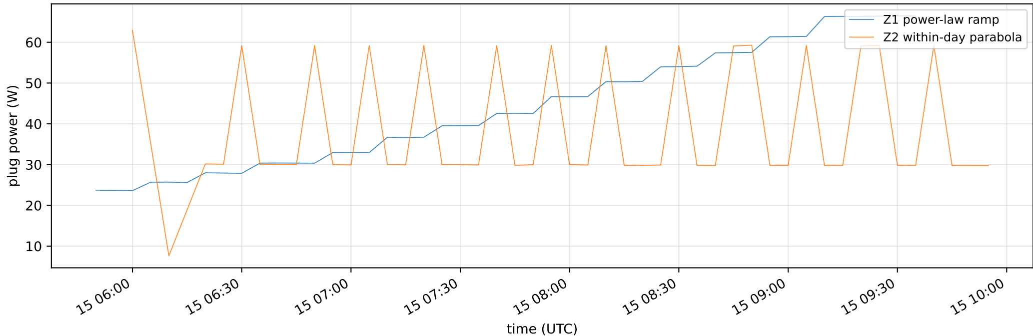
E18/P0.2 — plug power per zone
