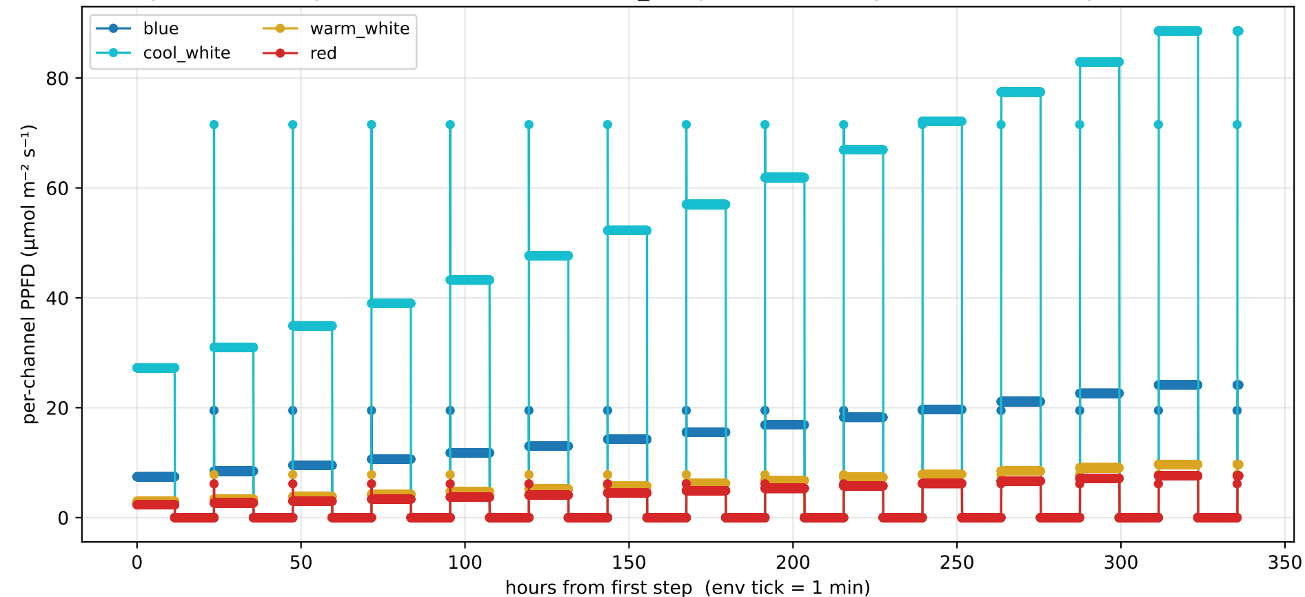
Z1 power-law ramp — actions emitted via main_real path (14 sim-days at 1-min env steps, 20160 total)
